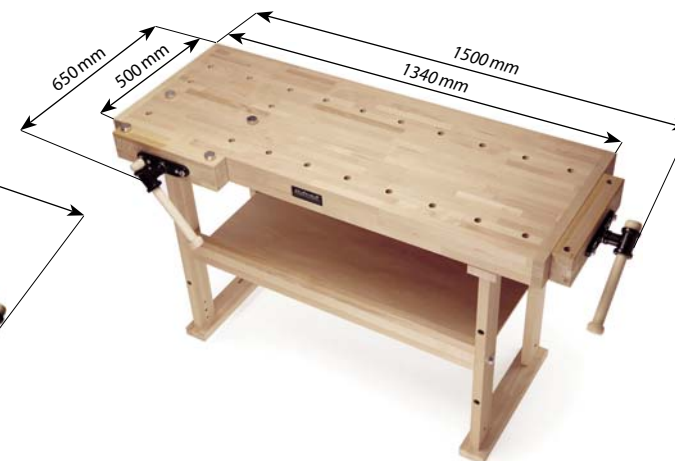
MEDIUM version of ADVANCED workbench MITTEL Version der ADVANCED Werkbank
