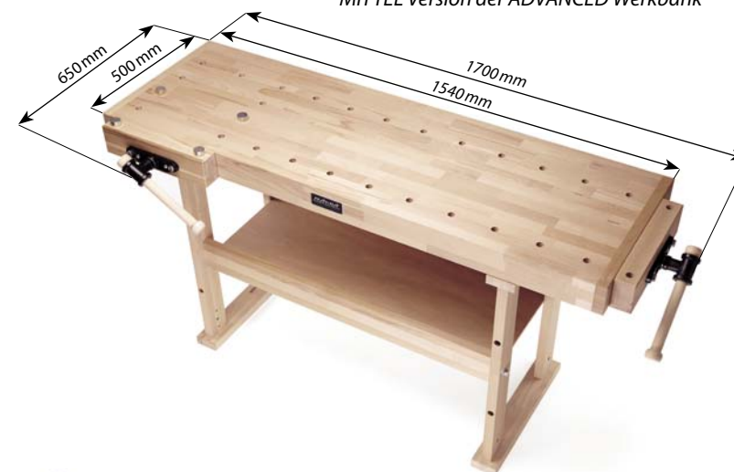
MEDIUM version of ADVANCED workbench MITTEL Version der ADVANCED Werkbank
